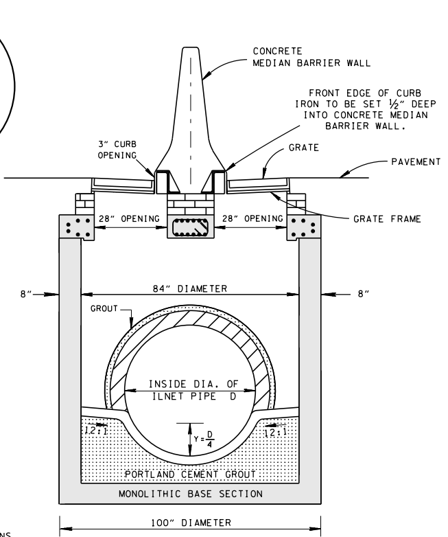
SECTION B-B
